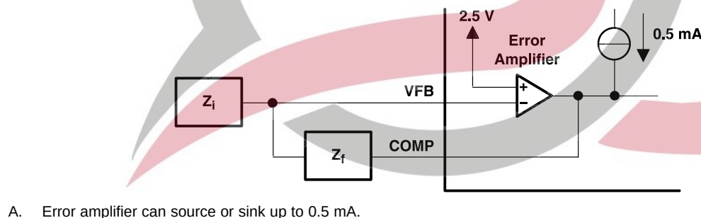
Figure 15. Error-Amplifier Configuration Schematic
